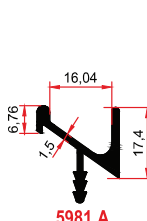
5981 A 0,300 Kg/m
