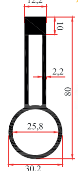
PRF-30538 1,340 Kg/m
